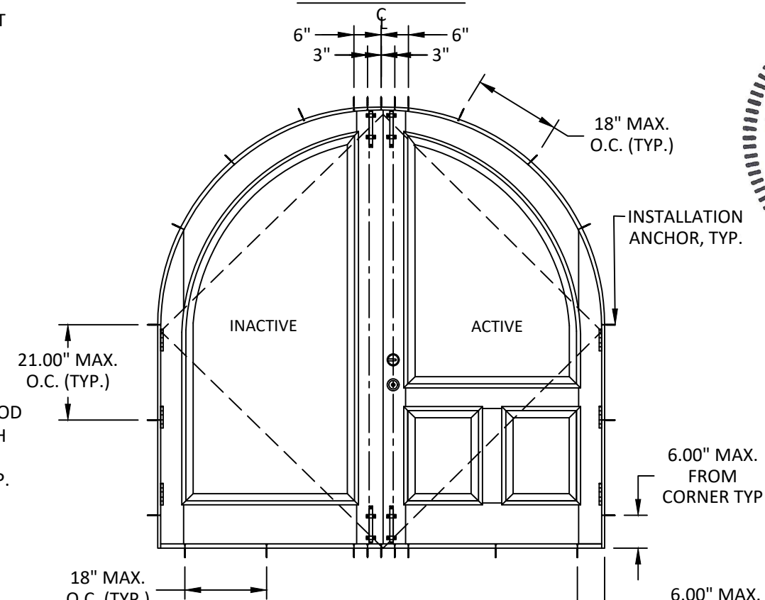
ANCHOR LAYOUT
