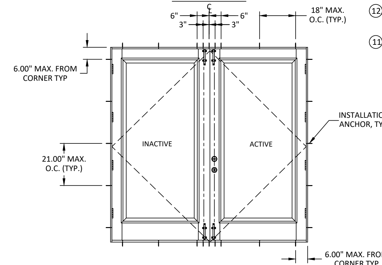
ANCHOR LAYOUT
